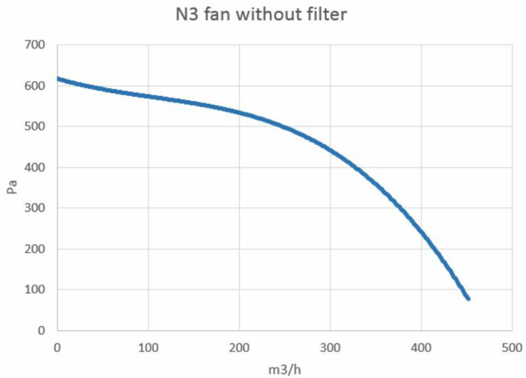
Pressure diagram
